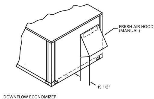
Figure 18. Fresh air hood (downflow units)
