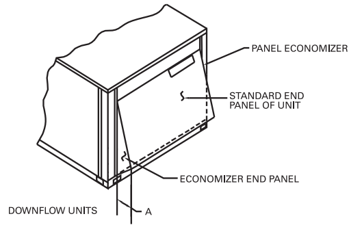
Figure 22. Economizer—downflow units
