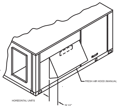
Figure 17. Fresh air hood (horizontal units)
