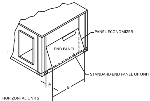
Figure 21. Economizer—horizontal units
