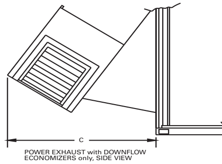
Figure 20. Power exhaust—downflow economizers—side view
