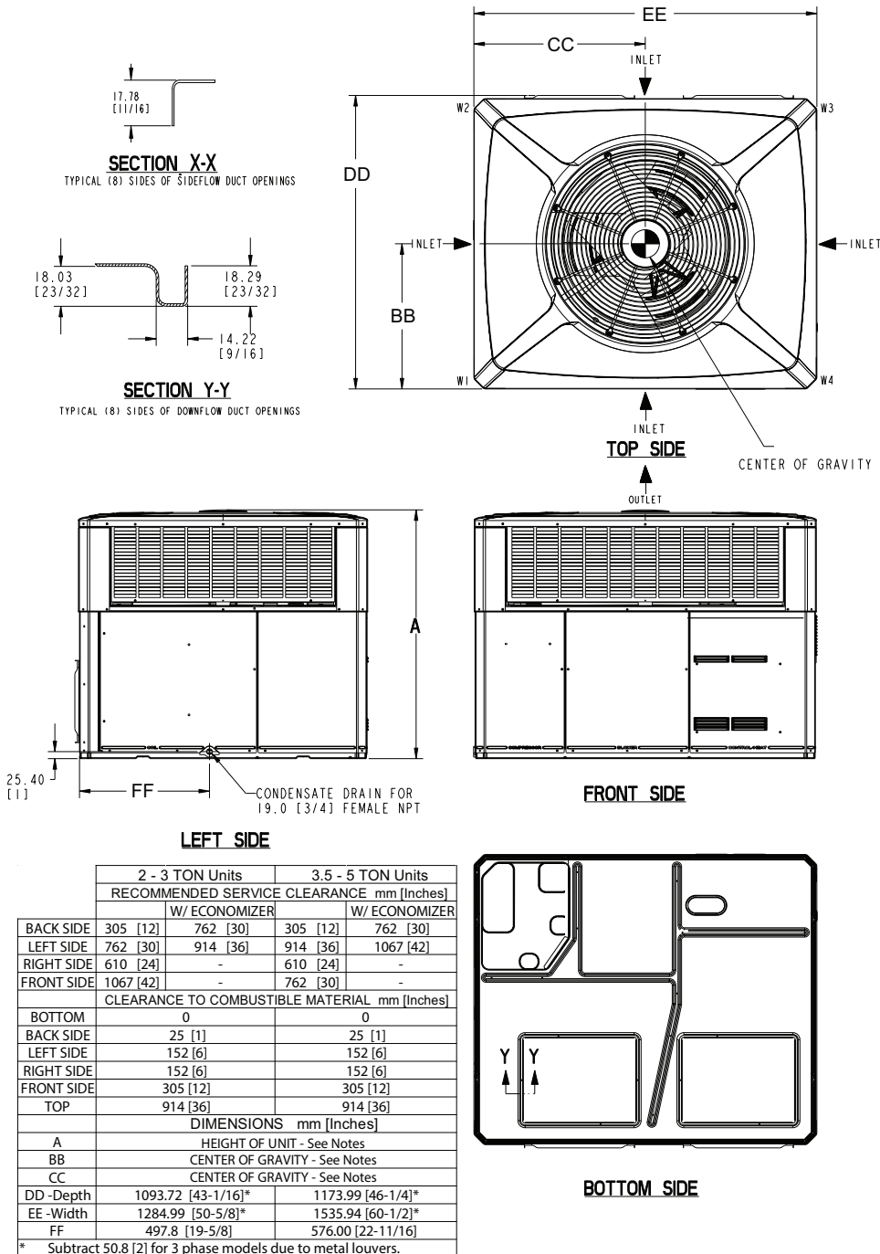
Figure 17. Space on sides requirements
